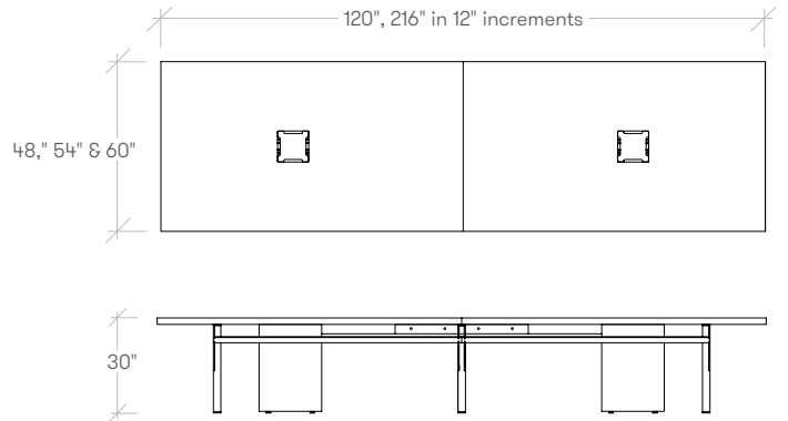
Two piece X-Leg Table - ZXDT
