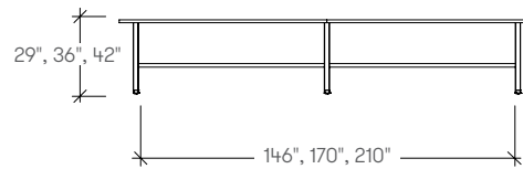
Rec Ganged Split Top Workshop Table (STMC)
