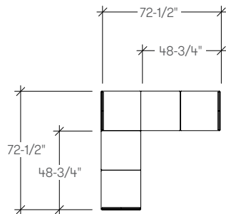
Five-Seat Bench, Left No Back (STP5C)
