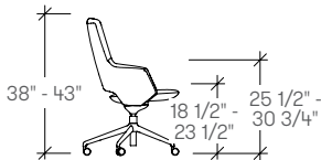
Jima Chair, Five-Star Task Base High Back (ARJCH)
