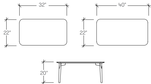
Havn Rectangular Occasional Table (STNL)
