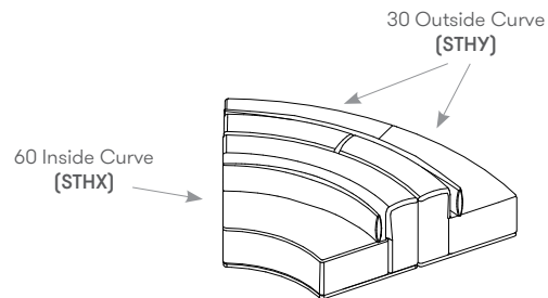
Two 30 Outside Curve units pair with one 60 Inside Curve Unit
