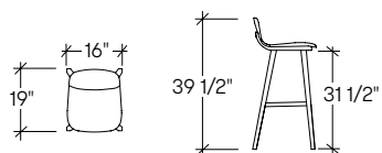
Bar Stool [ALKSB]
