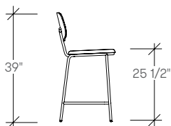
Santé Stool, Counter Height (TKAB2)
