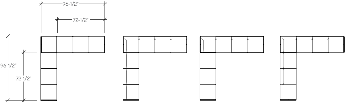
Seven-Seat Bench, Left No Back (STP7C)
