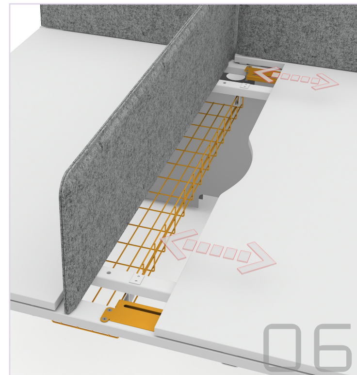
05 optional accessory beam 06 cable basket (with optional sliding top feature)
