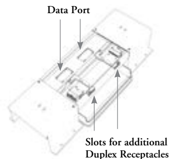
Bottom View Multi Circuit Table Power Module An additional 2 duplexes can be ordered and installed in the bottom sockets for extra power.
