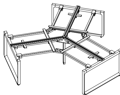
Three End Gables – Curve Open
