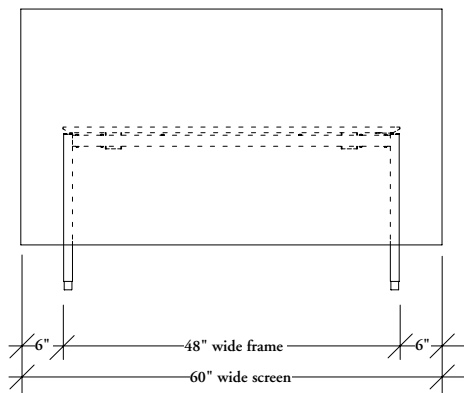
6" Overhang (WWCBSDG)
