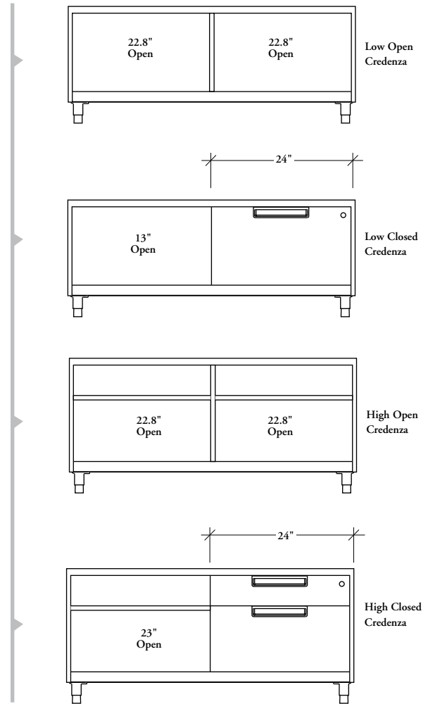
48" Width (all left shown for closed credenzas)
