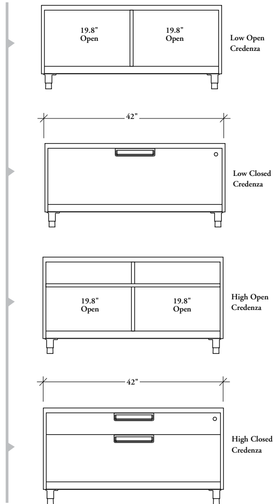
42" Width
