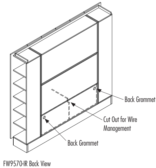
Standard Grommet Locations on Work Walls
