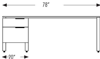
Single Pedestal Desk with Box/File installed flush.
