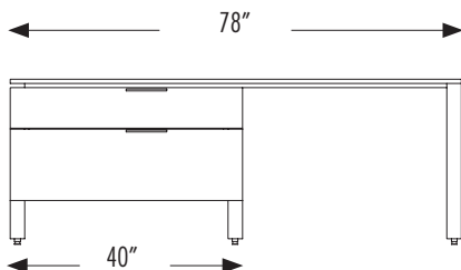
Single Pedestal Credenza with 40" Lateral Box/File installed flush.
