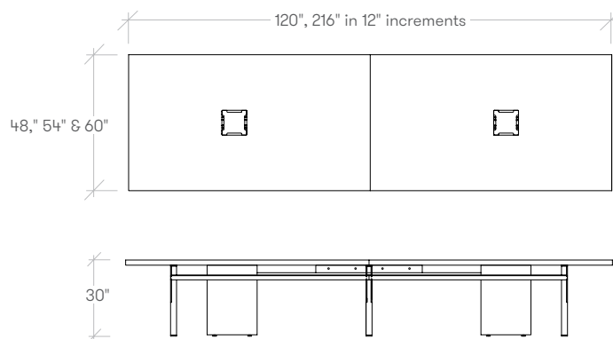
Two piece X-Leg Table - ZXDT
