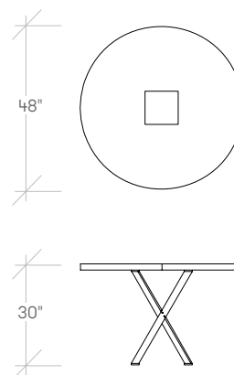
Small Table - ZRT
